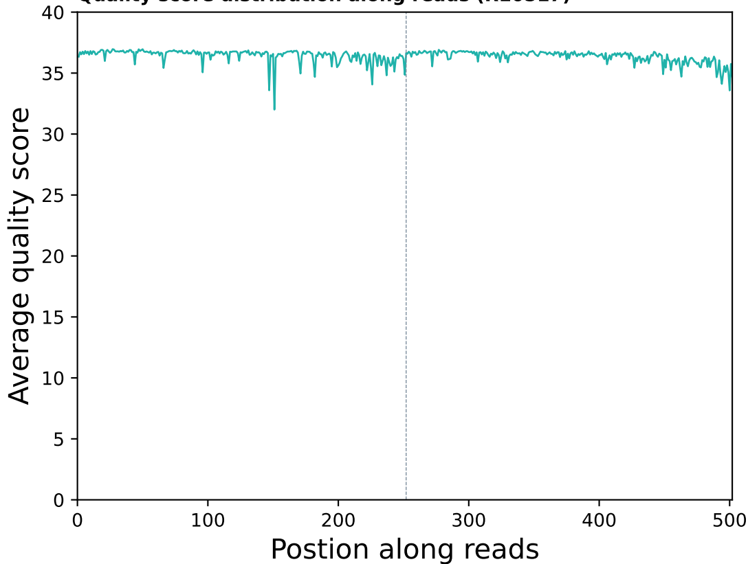
Quality score distribution along reads (R10517)
